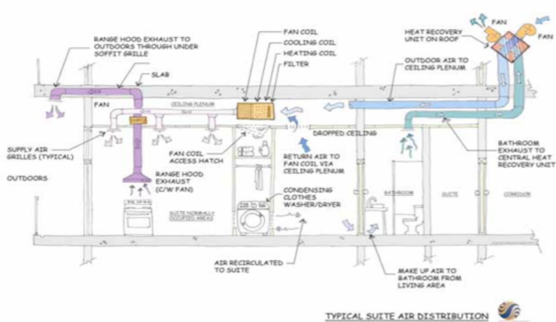
TYPICAL SUITE AIR DISTRIBUTION
