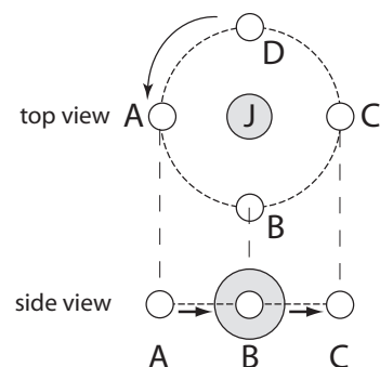
Figure 1: Jupiter's moons actual positions vs view from the Earth.
